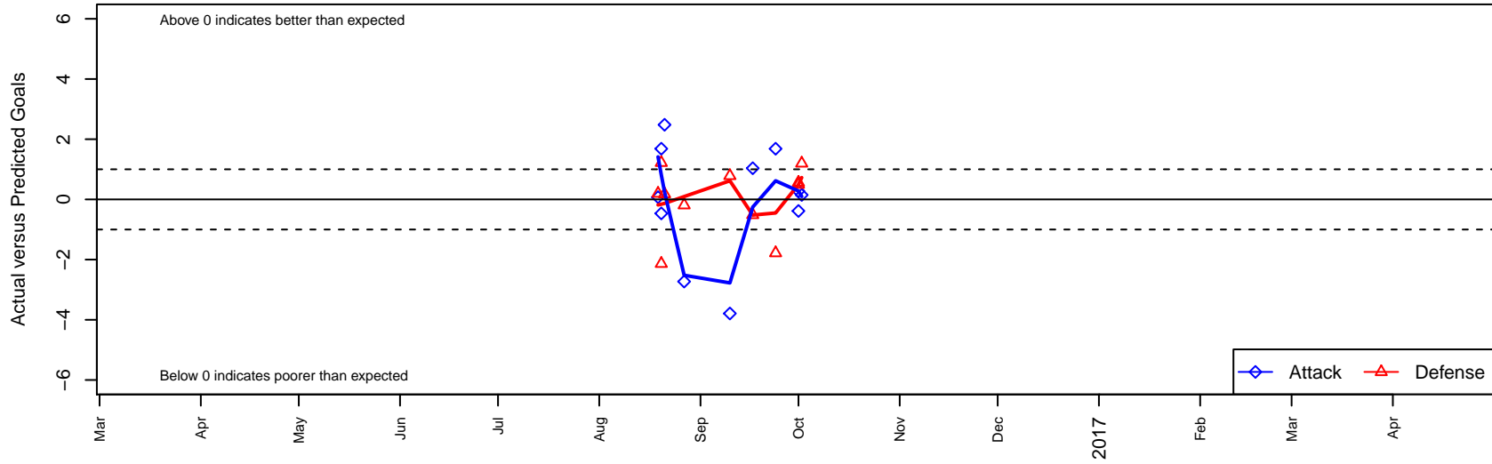
Idaho Rush Black G05 Dots are actual minus expected GF (blue circles) and GA (red triangles). Blue line is smoothed change in attack strength. Red is smoothed change in defense strength.
